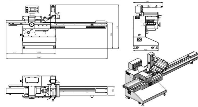
Machine Dimensions
